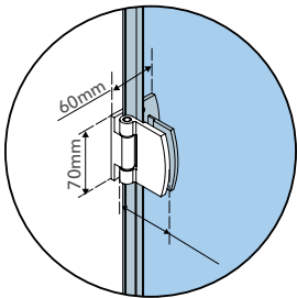
Bisagra pared-vidrio 90°
